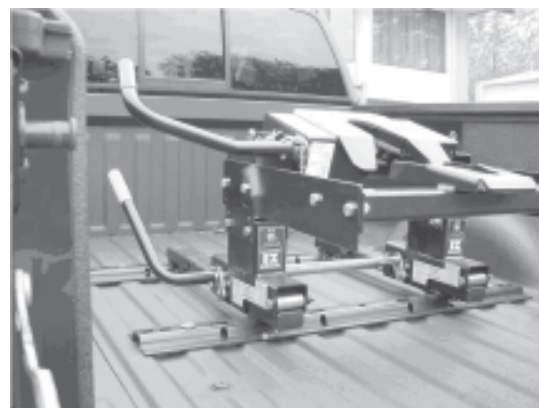
Figure 6-Complete Installation
