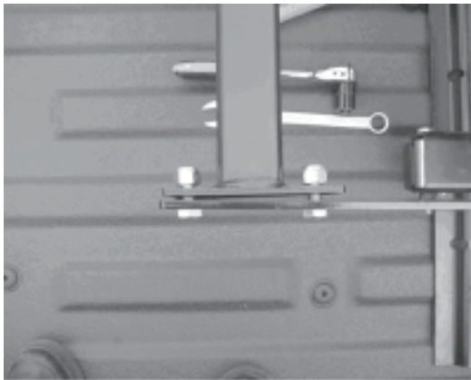
Figure 3-Cross Tube Attachment
