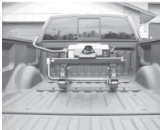
Figure 5-Complete Installation, Rear
